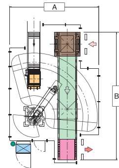
One Pallet Layout No. P01111
