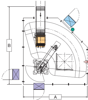
One Pallet Layout No. F01101
