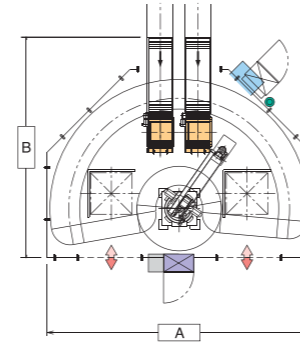
Two Pallets Layout No. F07202
