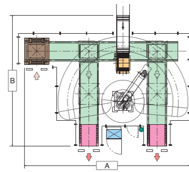
Two Pallets Layout No. P08122
